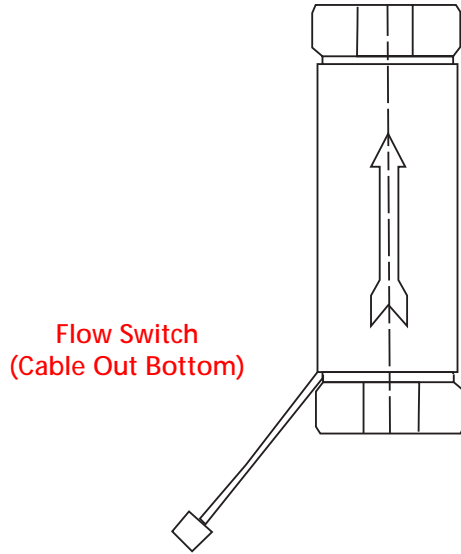
FIGURE 10. Flow Switch Configuration
