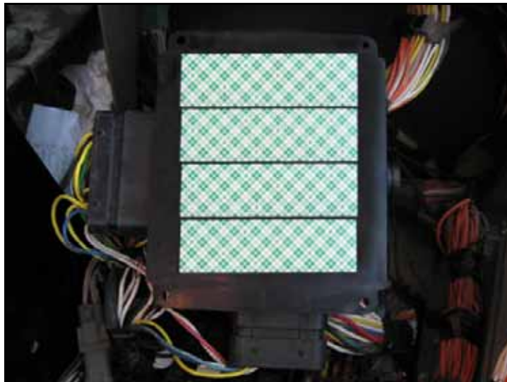
FIGURE 1. Double-Sided Tape on Case IH Interface Box
