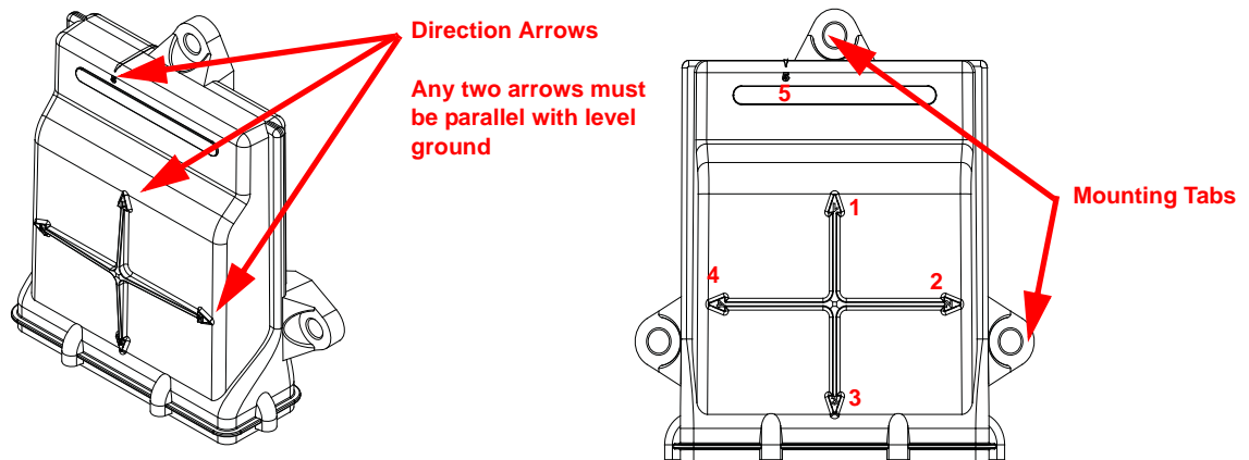
FIGURE 9. Node Mounting
