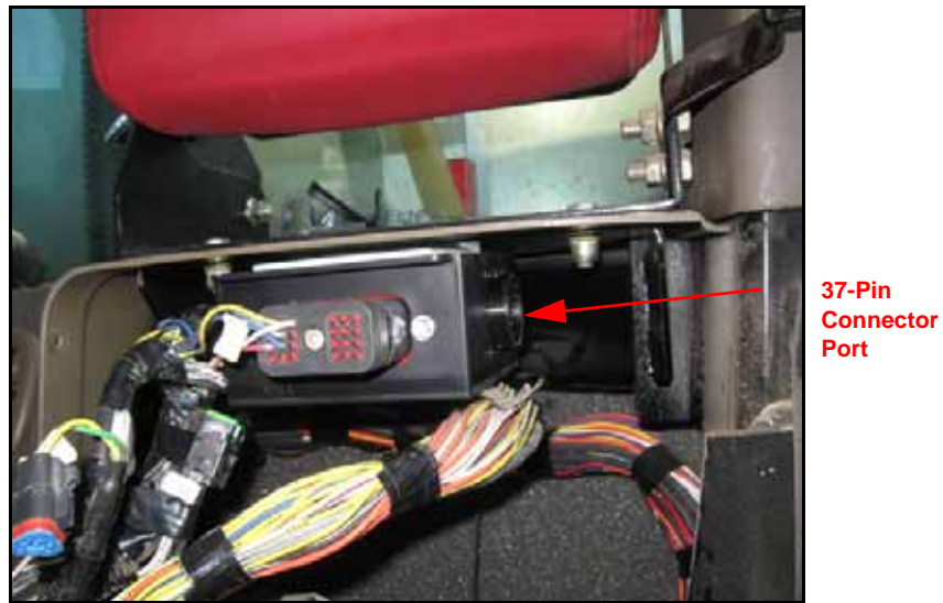
FIGURE 11. 37-Pin Connector Port Location
