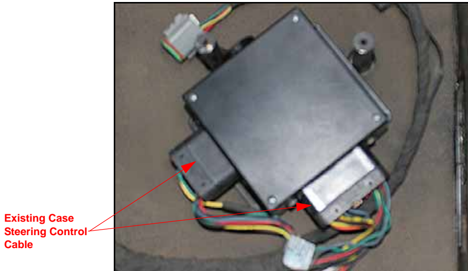
FIGURE 4. Case IH InterFace Cable Connected to the Case Interface Box
