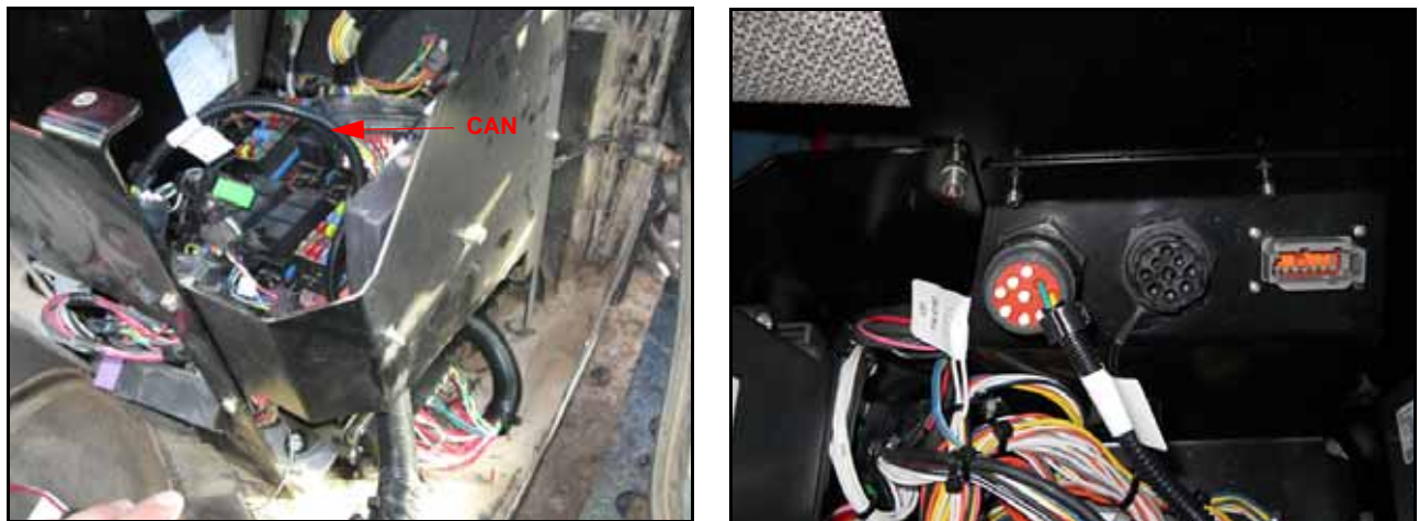
FIGURE 12. CAN Connector Installed on Machine's CAN System
