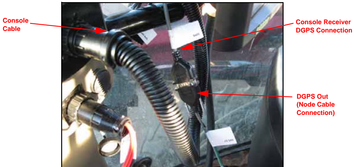
FIGURE 14. DGPS OUT Connected to Console Receiver Connection
