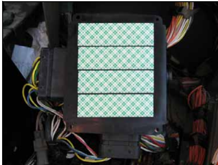
FIGURE 5. Double-Sided Tape on Case IH Interface Box
