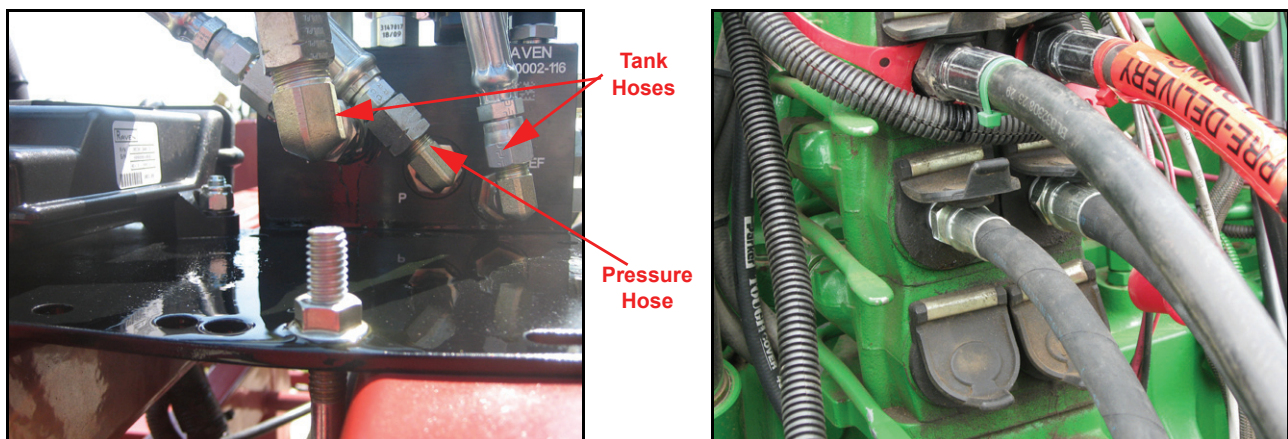
FIGURE 4. Pressure and Tank Hoses Installed
