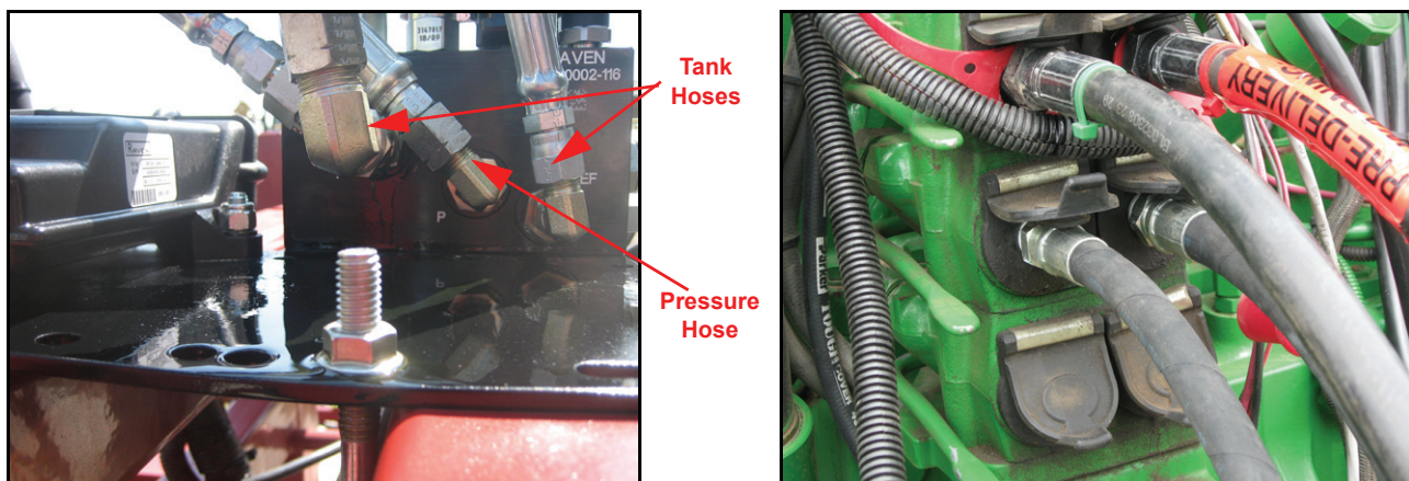
FIGURE 10. Pressure and Tank Hoses Installed
