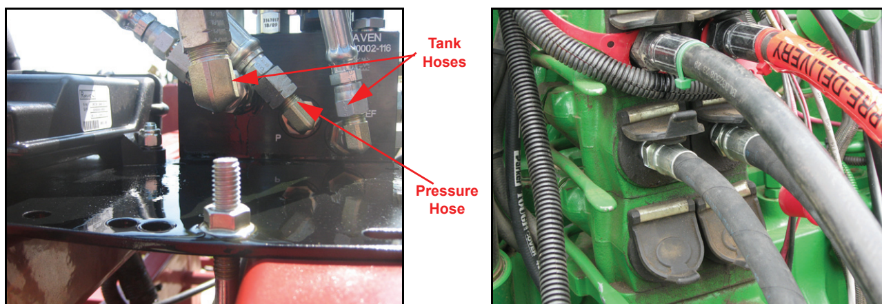
FIGURE 4. Pressure and Tank Hoses Installed
