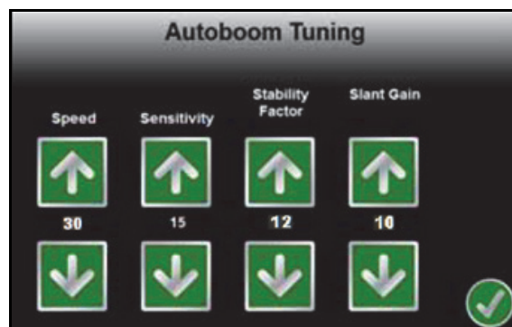
FIGURE 2. Envizio Pro Tuning Page with Default Settings for 120 ft. Boom
