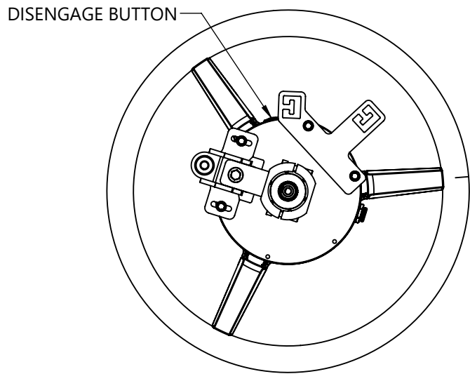
BOTTOM VIEW SCALE 1:6
