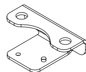
WHEEL SENSOR BRACKET, 63.5MM 107-8000-078
