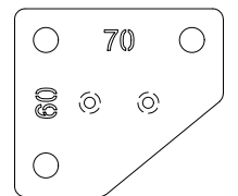
WHEEL SENSOR BRACKET, 60X70MM 107-8000-073
