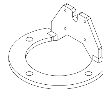
ANGLE SENSOR BRACKET, 3CM STEP 107-8000-067
