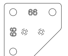
WHEEL SENSOR BRACKET, 66X66MM 107-8000-075
