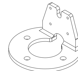
ANGLE SENSOR BRACKET, DEWULF OFFSET HARVESTER, FRONT 105MM 116-8000-030
