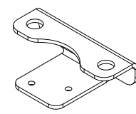
WHEEL SENSOR BRACKET, 73.5MM 107-8000-080
