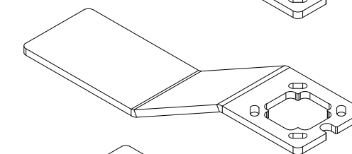
ANGLE SENSOR BRACKET, 5CM STEP 107-8000-068
