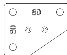
WHEEL SENSOR BRACKET, 60X80MM 107-8000-074
