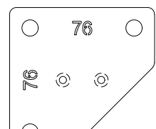
WHEEL SENSOR BRACKET, 76X76MM 107-8000-076
