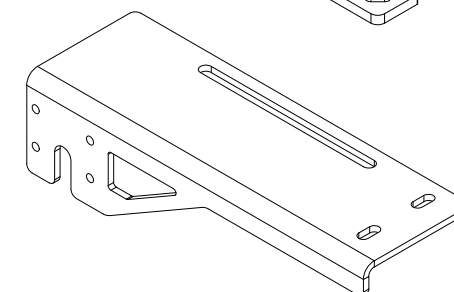
ANGLE SENSOR BRACKET, SIDESHIFT IMPLEMENT FRAME 107-8000-086
