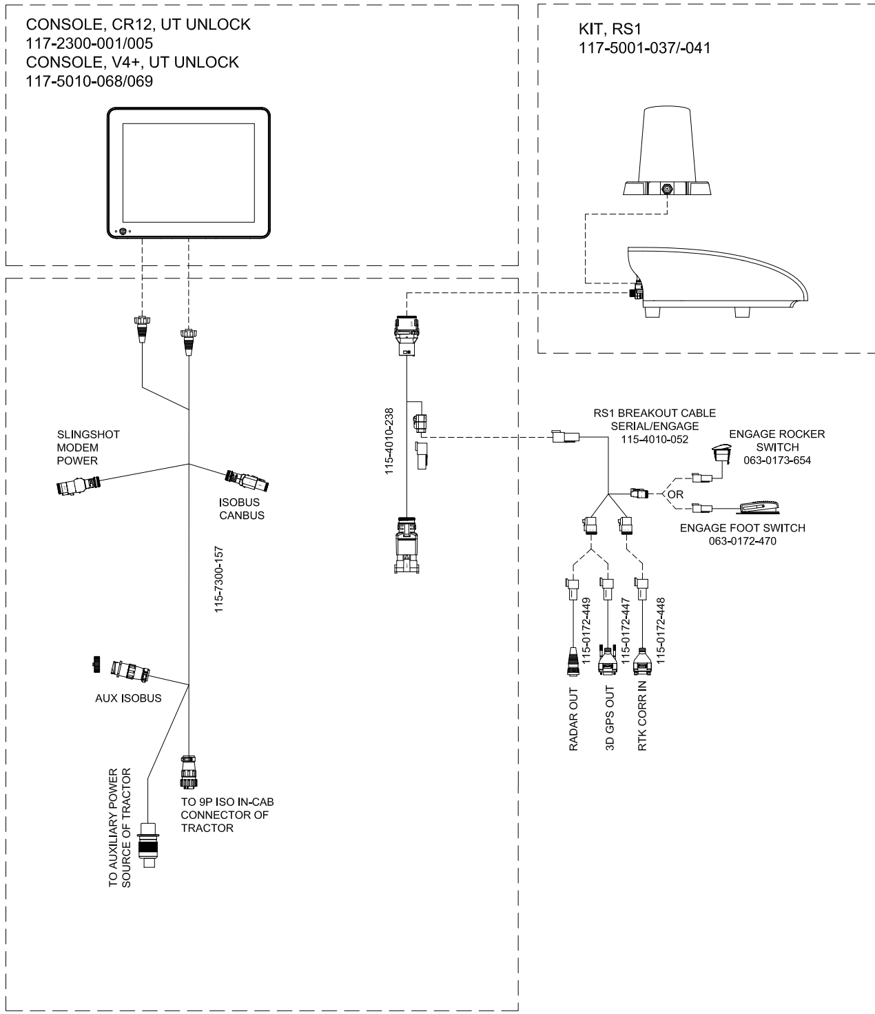
FIGURE 11. RS1 (with CR12) System Drawing for McCormick X7/X8(P/N 054-5038-006 Rev. A)
