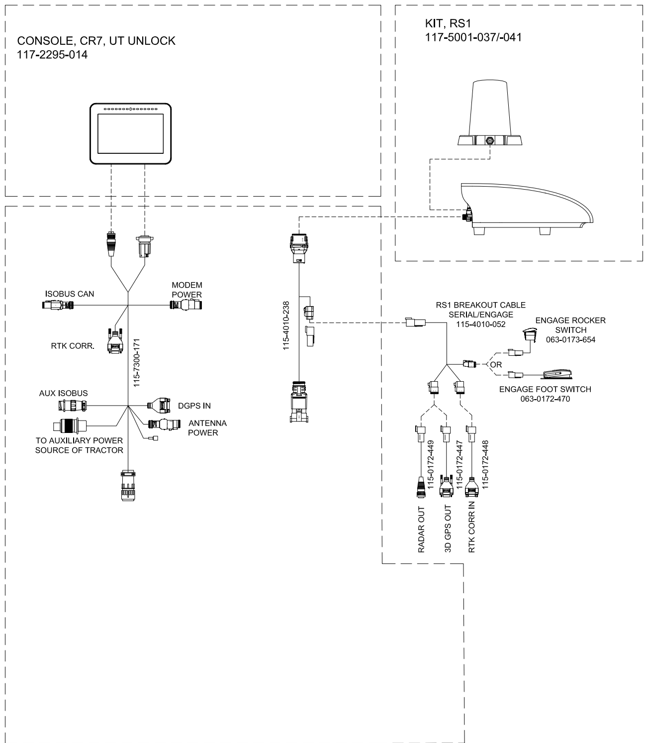
FIGURE 10. RS1 (with CR7) System Drawing for McCormick X7/X8 (P/N 054-5038-005 Rev. A)
