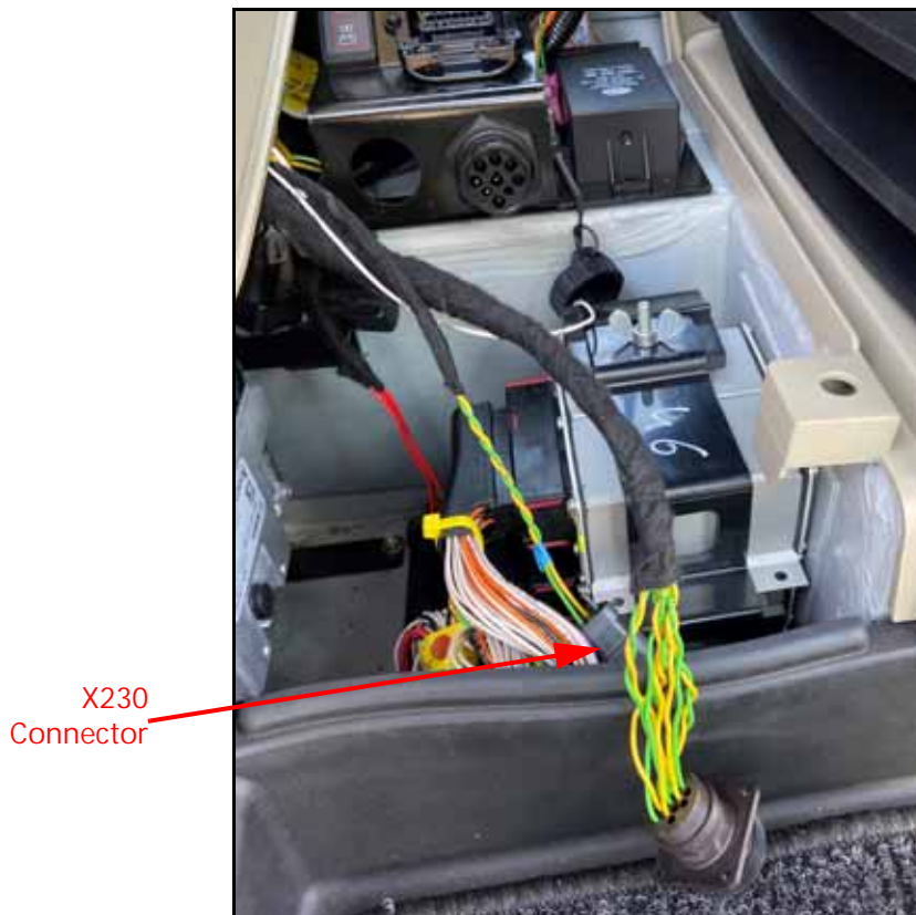
FIGURE 3. X230 Connector Location
