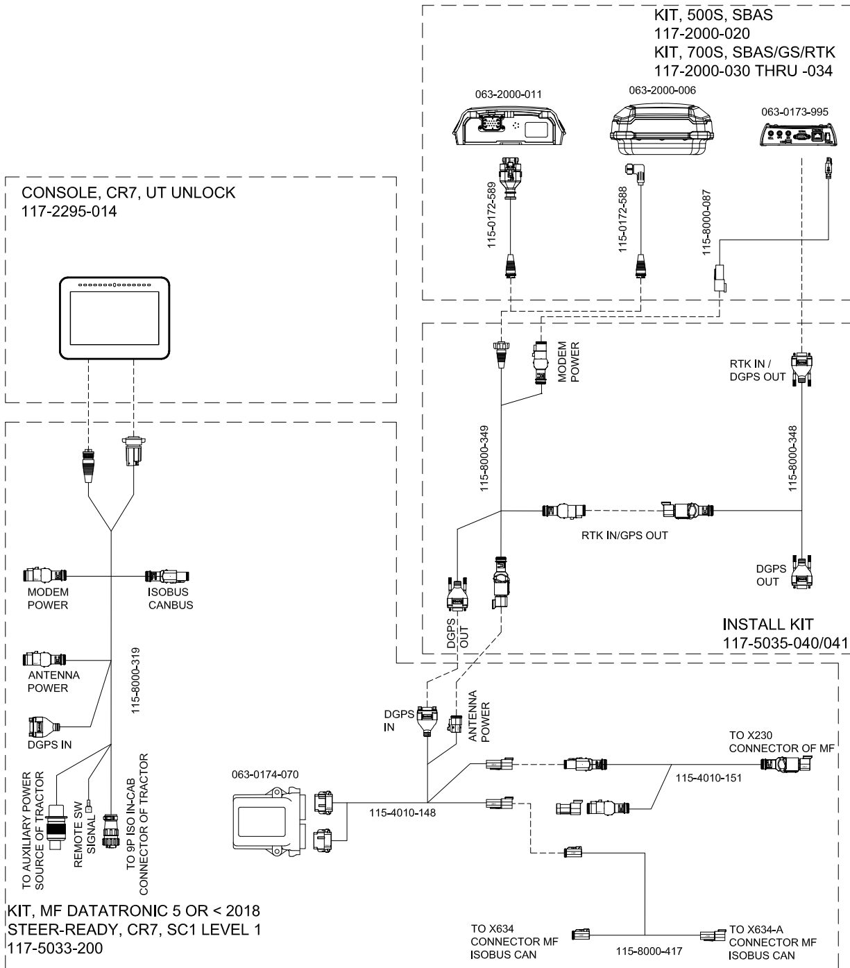
FIGURE 17. System Drawing, MF Datatronic 5 or < 2018 Steer-Ready, CR7, SC1 (P/N 054-5033-200 Rev. A)
