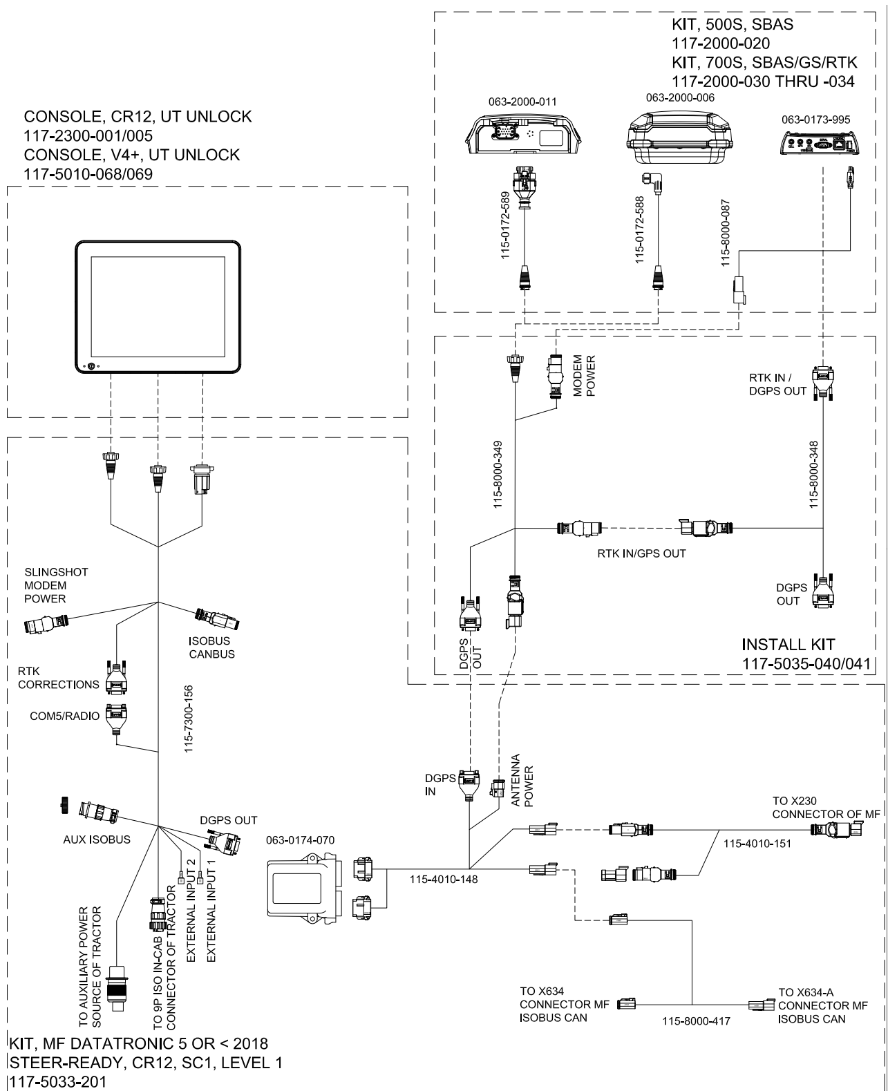
FIGURE 18. System Drawing, MF Datatronic 5 or < 2018 Steer-Ready, CR12, SC1 (P/N 054-5033-201 Rev. A)
