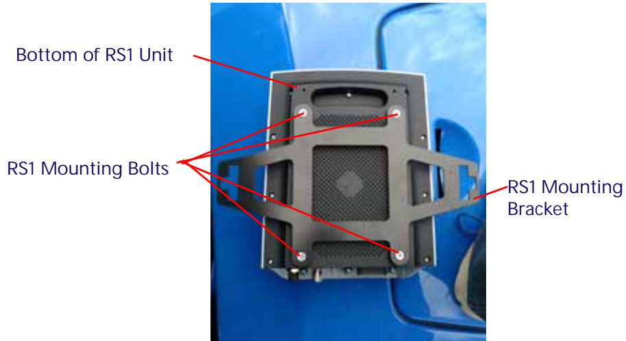
FIGURE 1. RS1 Mounted to Bracket
