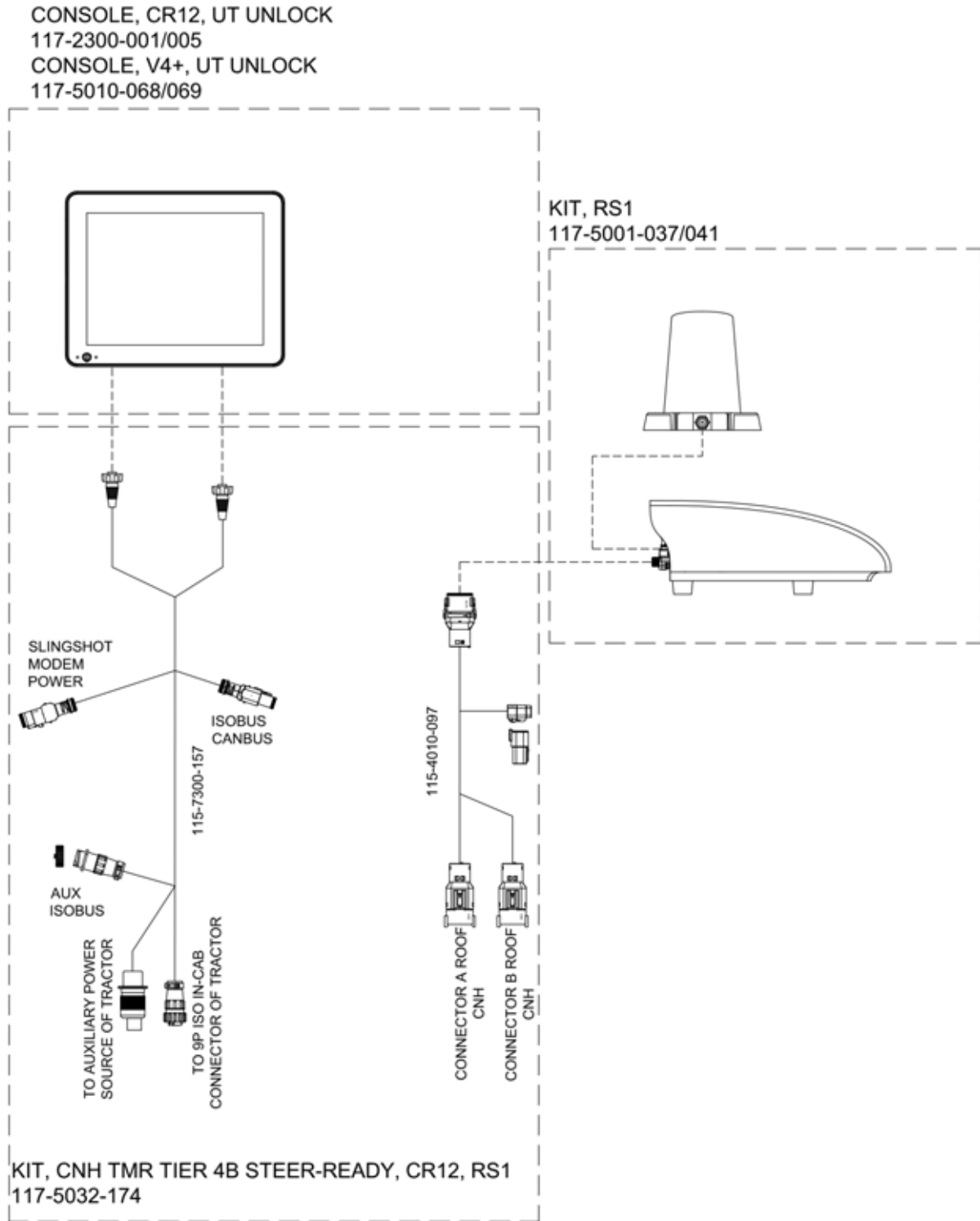
FIGURE 12. CNH, TMR TIER 4B Steer-Ready CR12 & RS1 System Drawing (P/N 054-5032-174)
