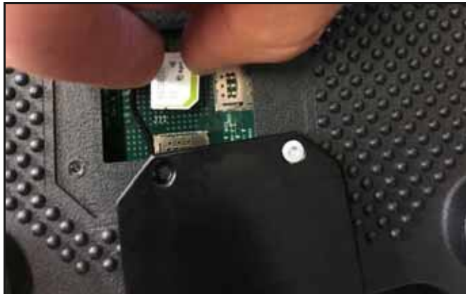
FIGURE 5. SIM Card Inserted in SIM Slot
