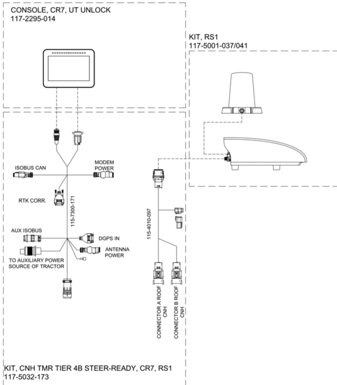
FIGURE 11. CNH, TMR TIER 4B Steer-Ready, CR7 & RS1 System Drawing (P/N 054-5032-173)
