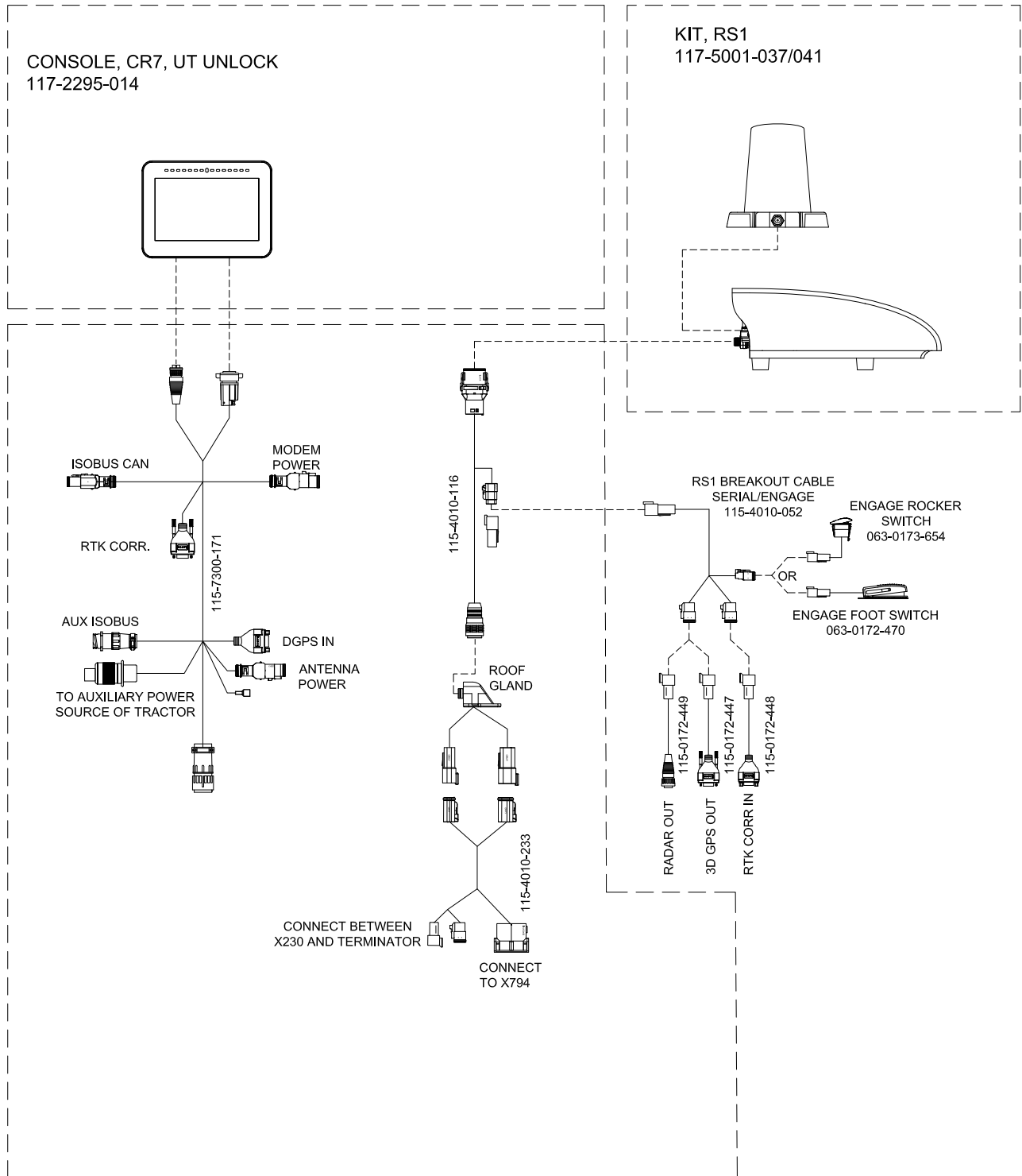
FIGURE 18. RS1™ with CR7™ for Massey Ferguson Autoguide-ready System Drawing (P/N 054-5033-265 Rev. A)
