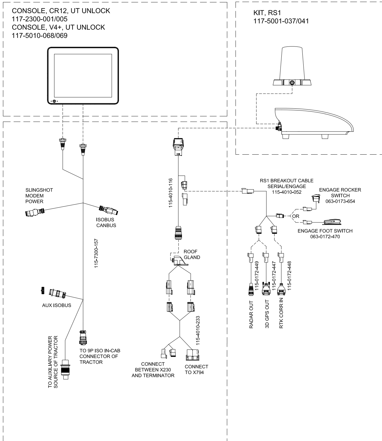
FIGURE 19. RS1™ with CR12™ for Massey Ferguson Autoguide-ready System Drawing (P/N 054-5033-266 Rev. A)
