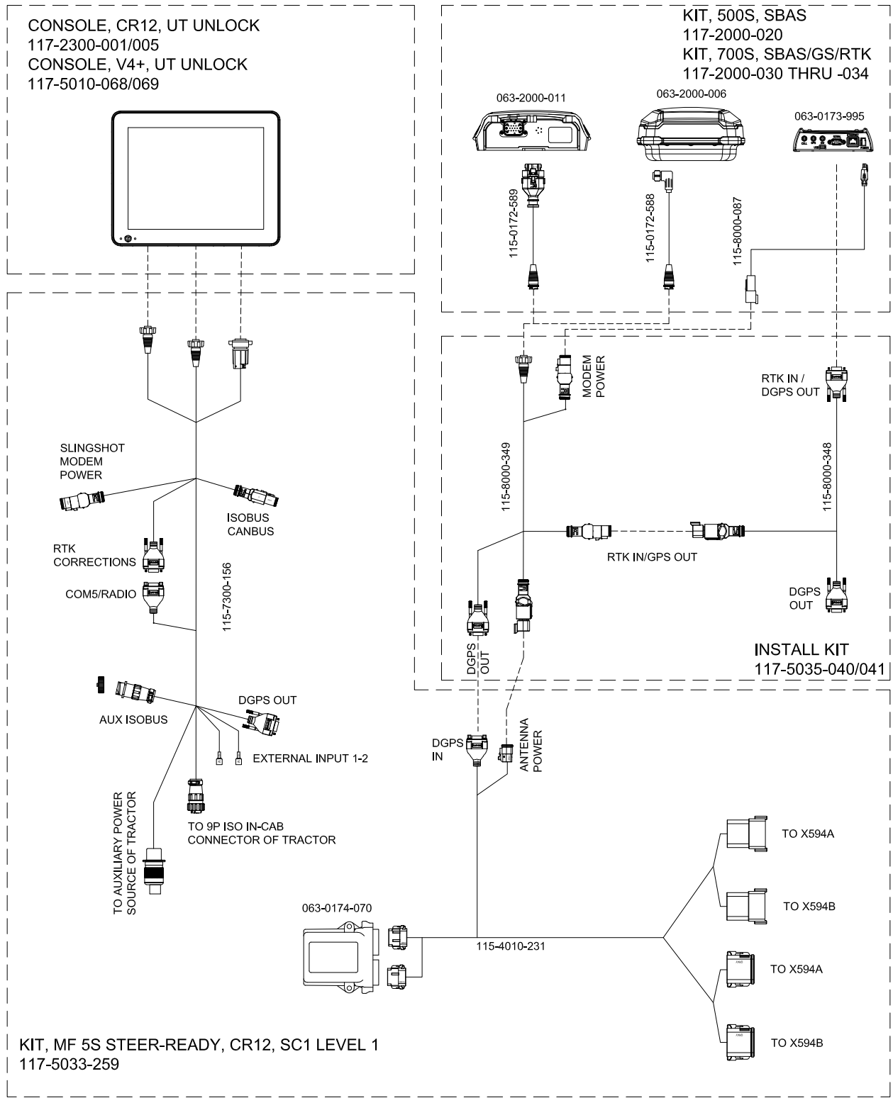
FIGURE 17. MF 5s CR12 & TC1 System Drawing (P/N 054-5033-259 Rev. A)
