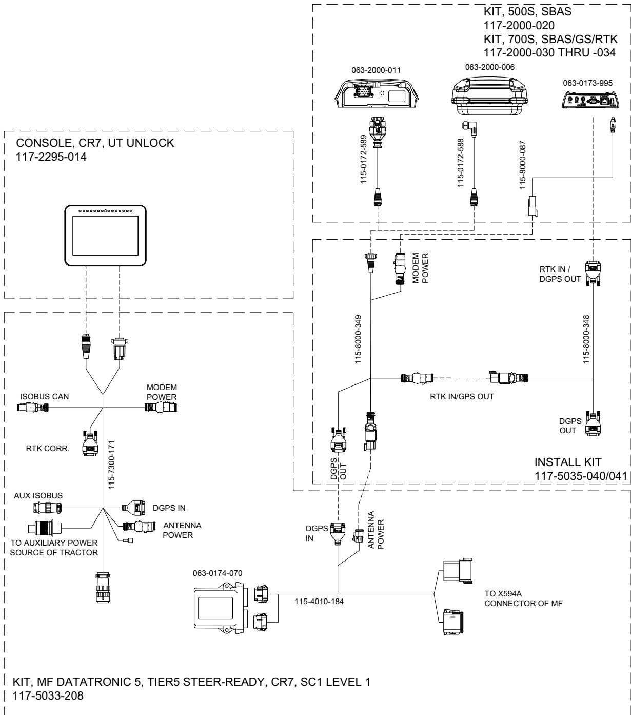
FIGURE 16. MF Datatronic 5 Tier 5 Steer-Ready CR7 & SC1 System Drawing (P/N 054-5033-208 Rev. C)
