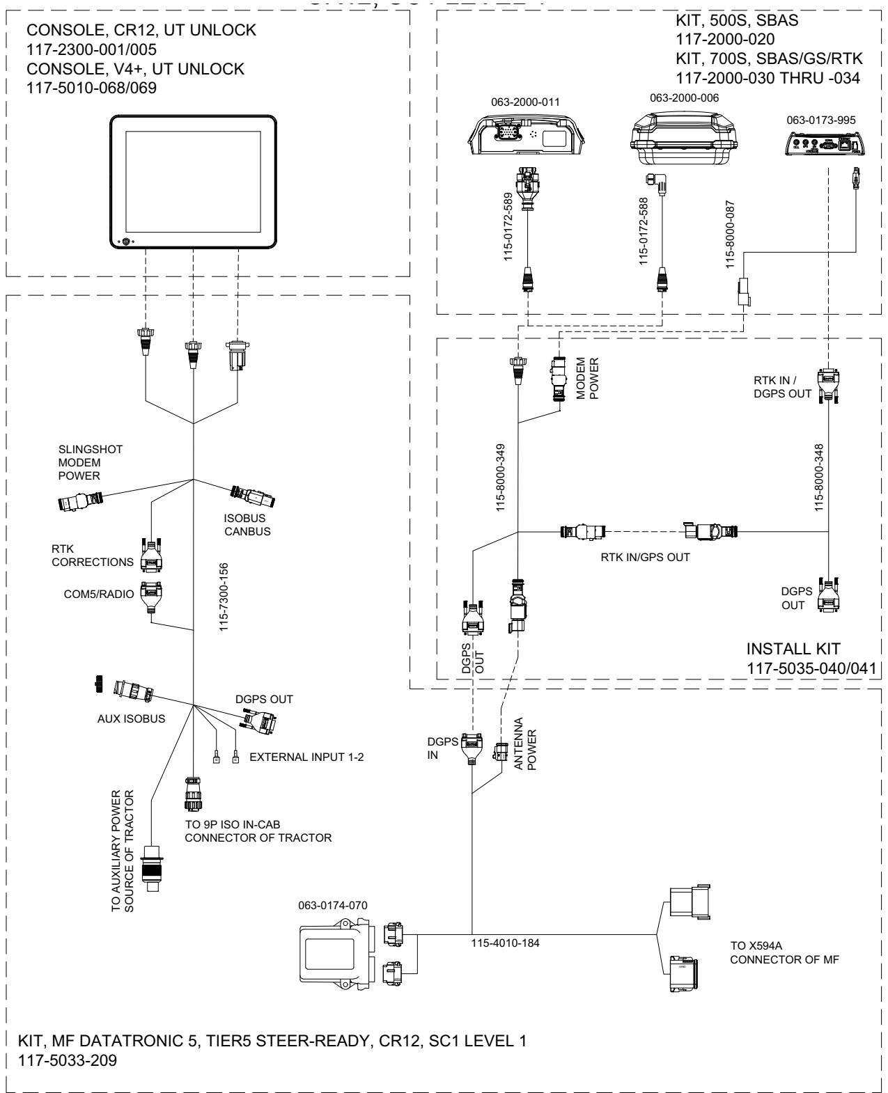
FIGURE 17. MF Datatronic 5 Tier 5 Steer-Ready CR12 & SC1 System Drawing (P/N 054-5033-209 Rev. B)
