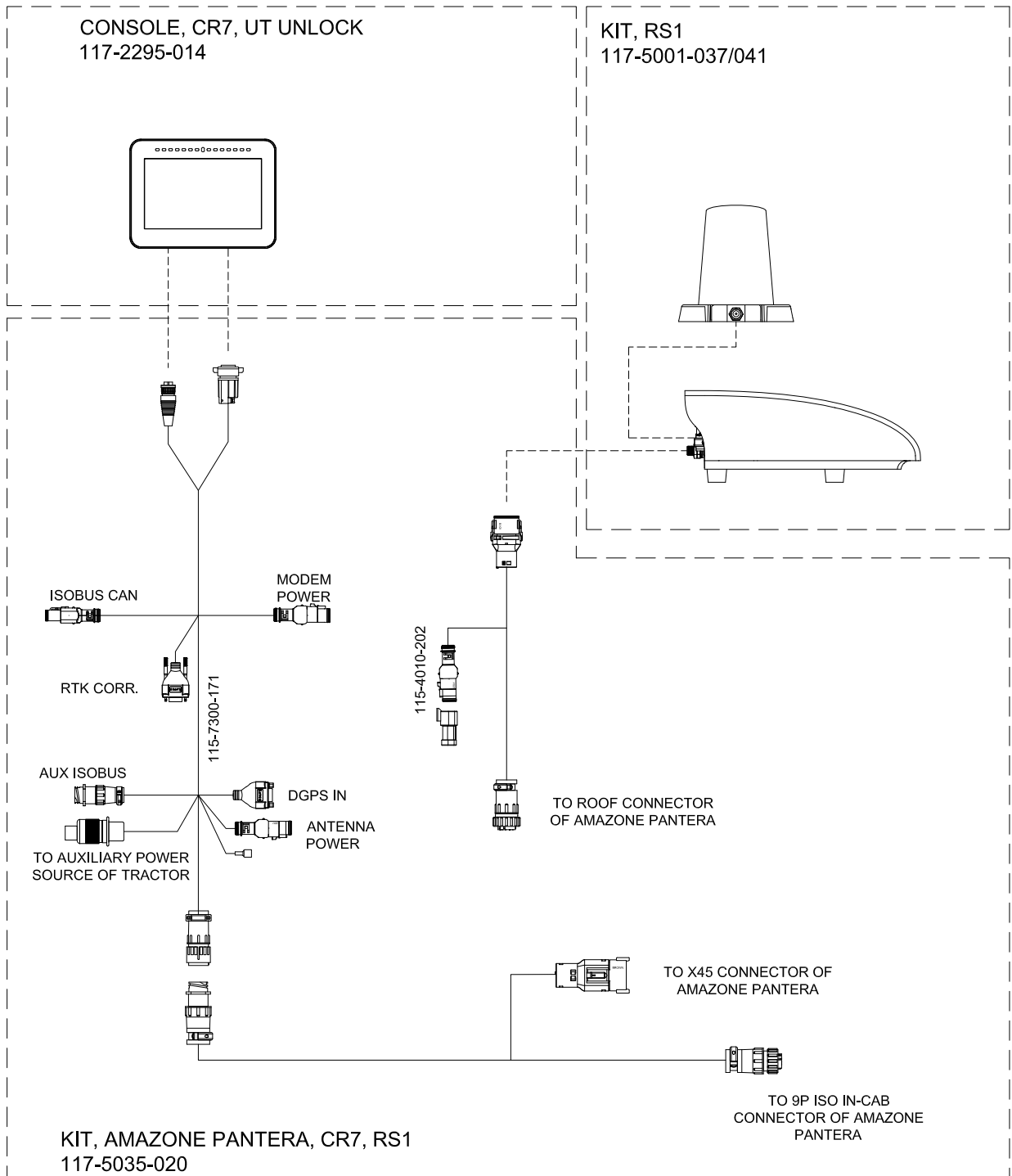
FIGURE 12. Amazone Pantera CR7 & RS1 System Drawing (P/N 054-5035-020 Rev. A)
