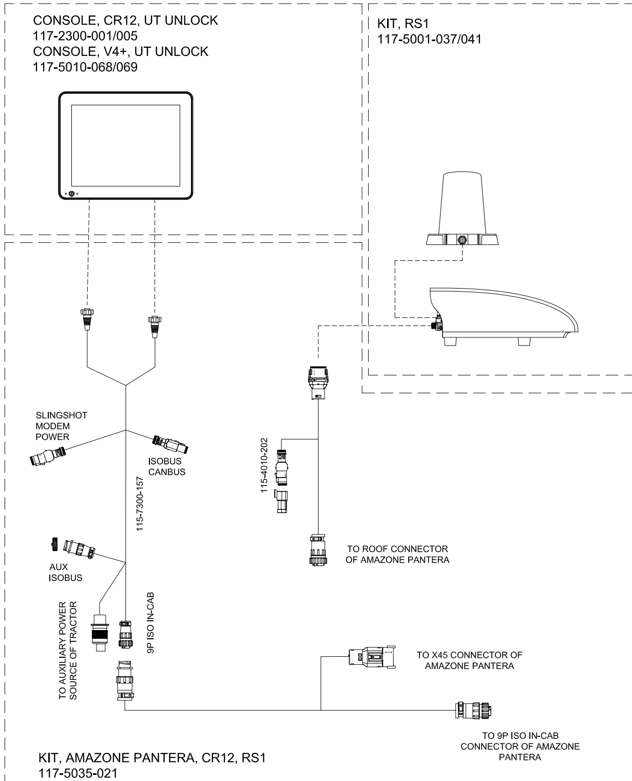
FIGURE 13. Amazone Pantera CR12 & RS1 System Drawing (P/N 054-5035-021 Rev. A)
