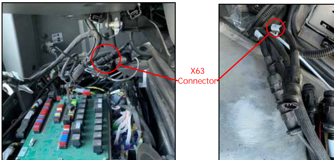
FIGURE 2. 9-Pin ISObus In-Cab Connector (Labeled X63)
