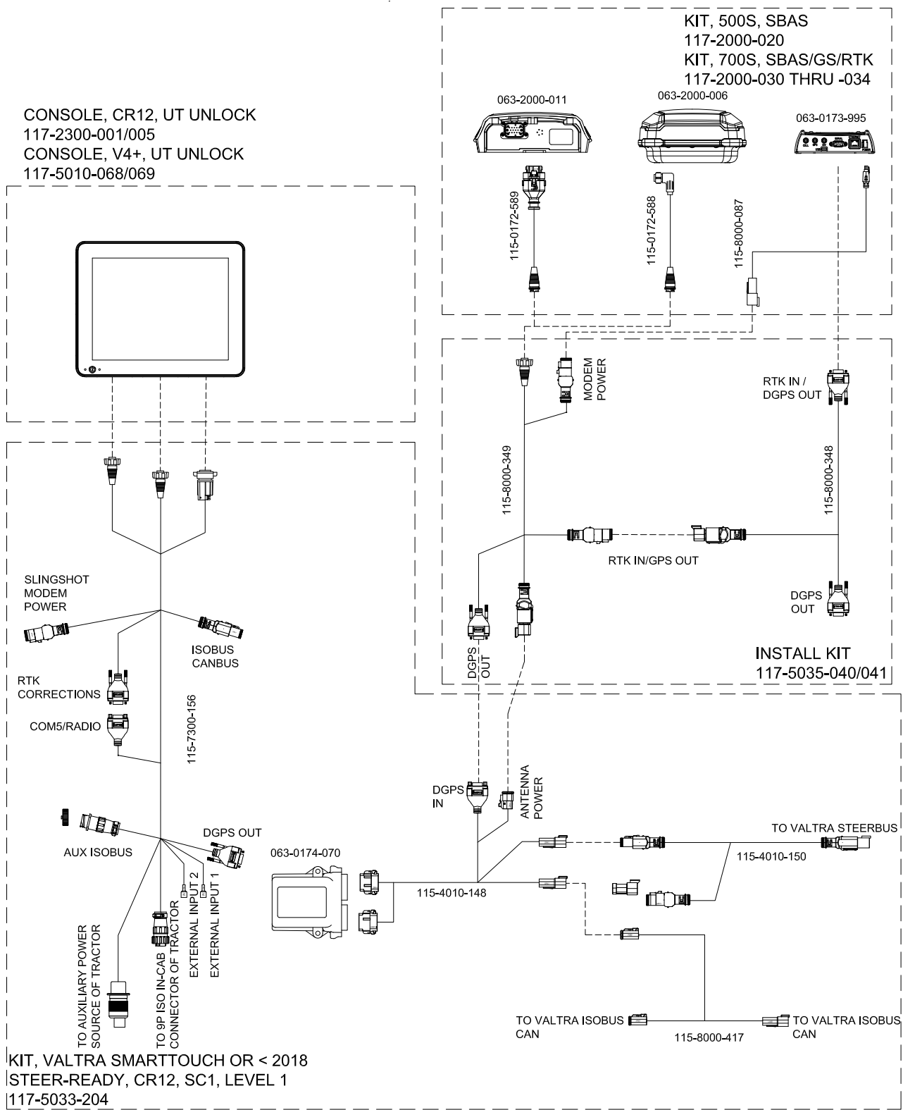
FIGURE 19. Valtra SmartTouch CR12 & SC1 System Drawing (P/N 054-5033-204 Rev. A)
