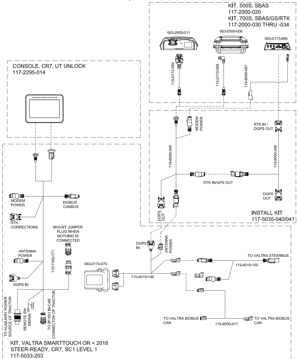
FIGURE 18. Valtra SmartTouch CR7 & SC1 System Drawing (P/N 054-5033-203 Rev. B)
