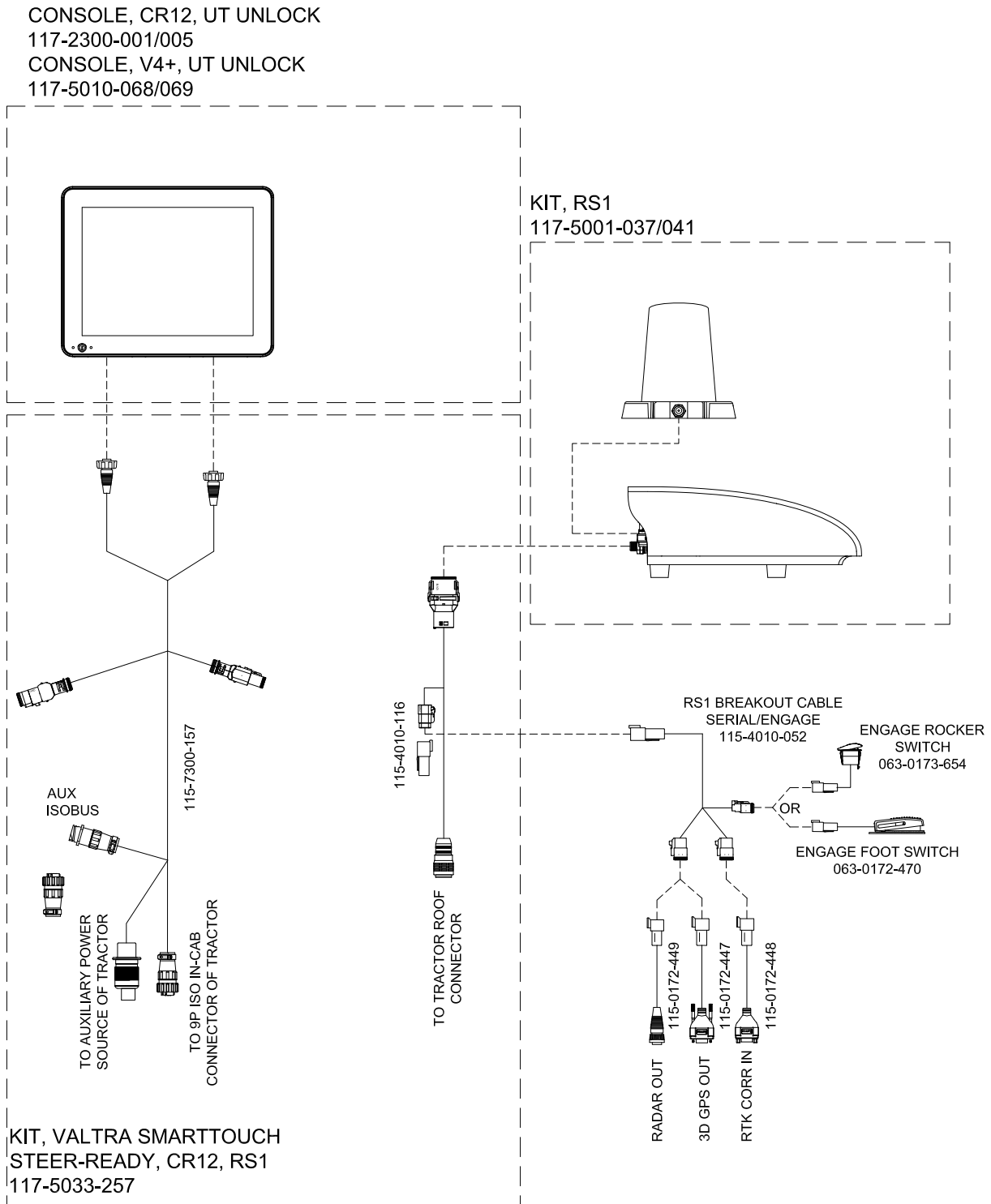
FIGURE 12. Valtra SmartTouch CR12 & RS1 System Drawing (P/N 054-5033-257 Rev. B)
