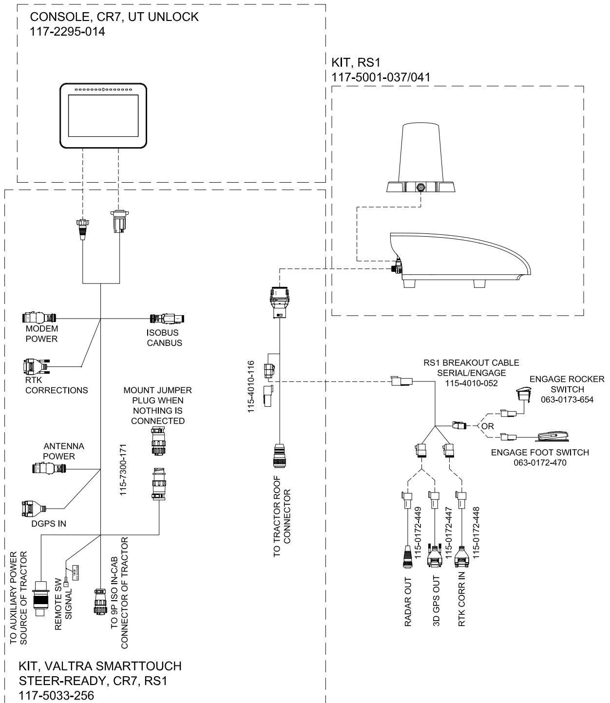
FIGURE 11. Valtra SmartTouch CR7 & RS1 System Drawing (P/N 054-5033-256 Rev. B)
