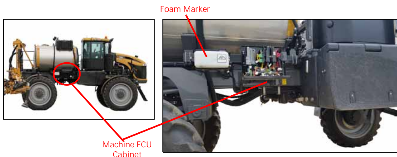
FIGURE 1. RoGator 1300 ECU Cabinet and Foam Marker Pump Location
