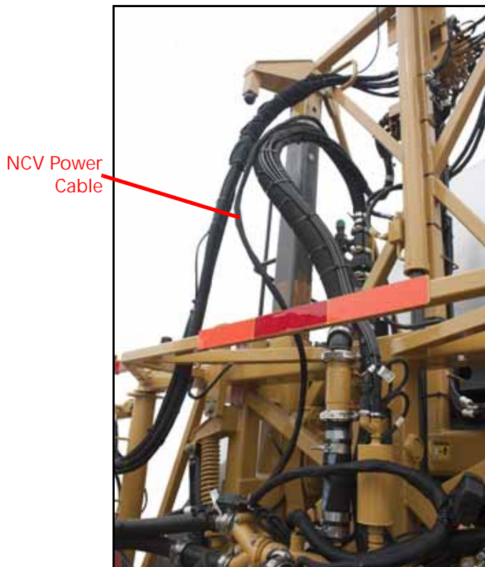
FIGURE 2. NCV Power Cable Center Rack Routing
