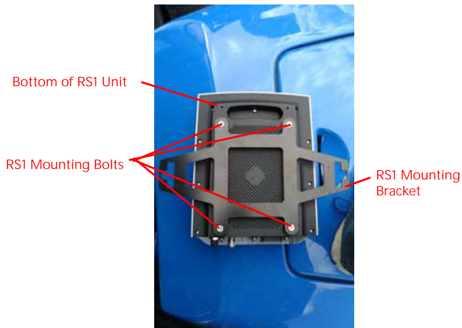
FIGURE 1. RS1 Mounted to Bracket
