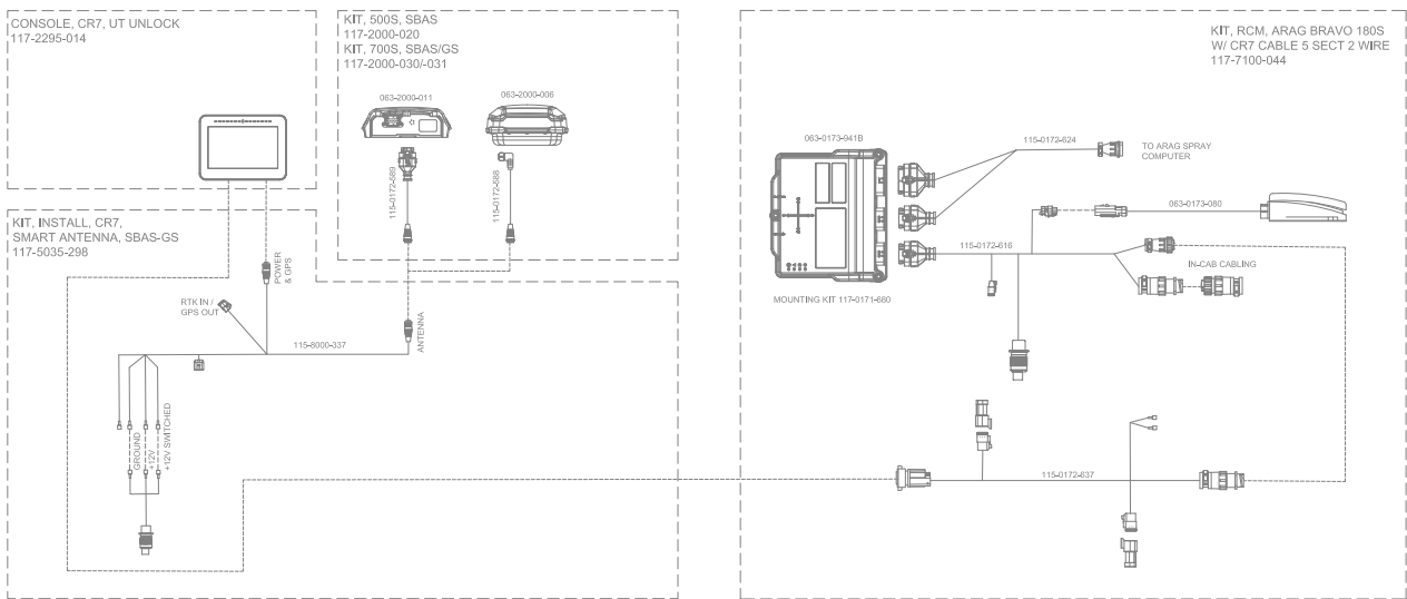
FIGURE 11. RCM ARAG, 5 Sections, 2-Wire Valve w/ CR7 ISO Cable System Drawing (P/N 054-7100-044 Rev. A)
