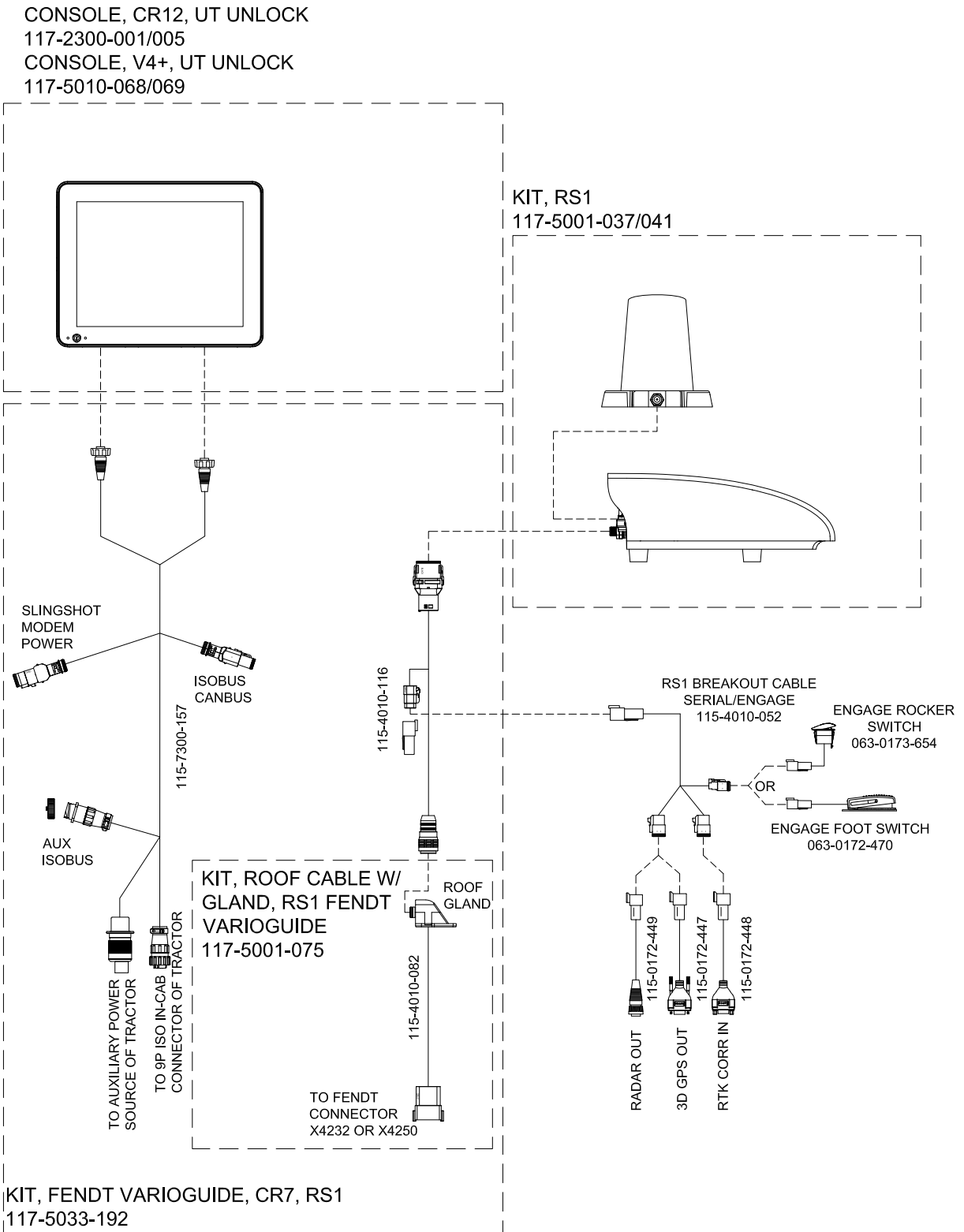
FIGURE 17. Fendt Varioguide CR12 & RS1 System Drawing (P/N 054-5033-193 Rev. A)
