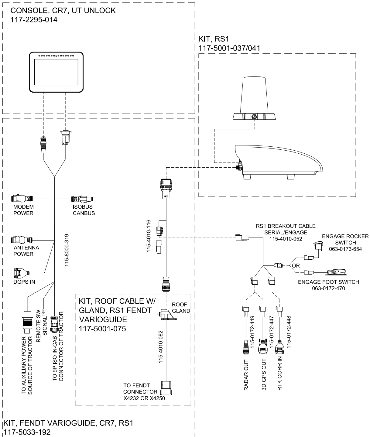
FIGURE 16. Fendt Varioguide CR7 & RS1 System Drawing (P/N 054-5033-192 Rev. A)
