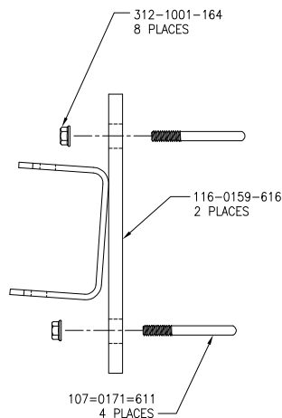
ULTRASONIC SENSOR MOUNTING BRACKET
