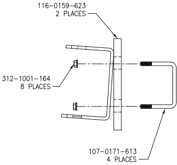
ULTRASONIC SENSOR MOUNTING BRACKET
