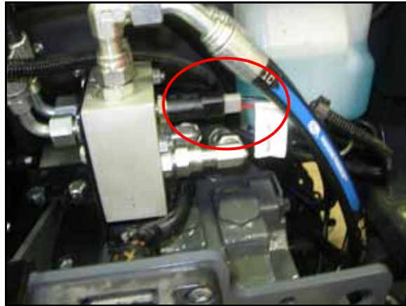
FIGURE 11. Pressure Transducer Connection
