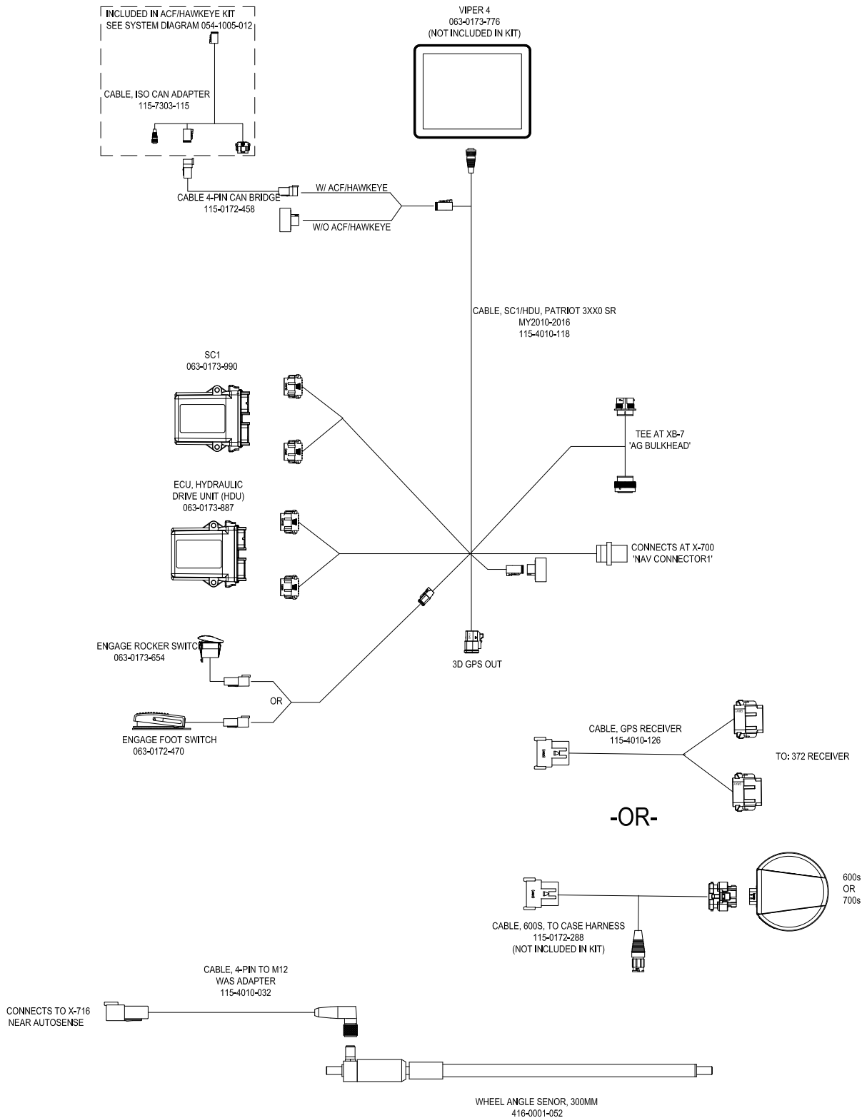
FIGURE 12. SC1/HDU Cabling for Case IH Patriot 3xxx (2010-2016, Steer Ready)
