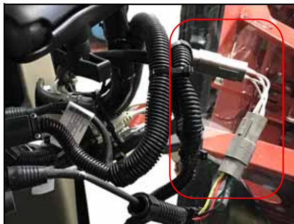
FIGURE 7. CAN Bridge Cable Connected to HDU Harness Cable
