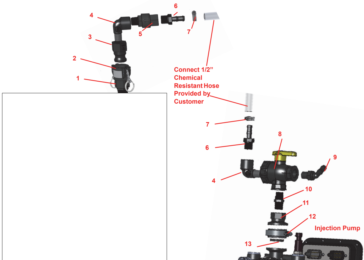
FIGURE 1. Top of Tank
