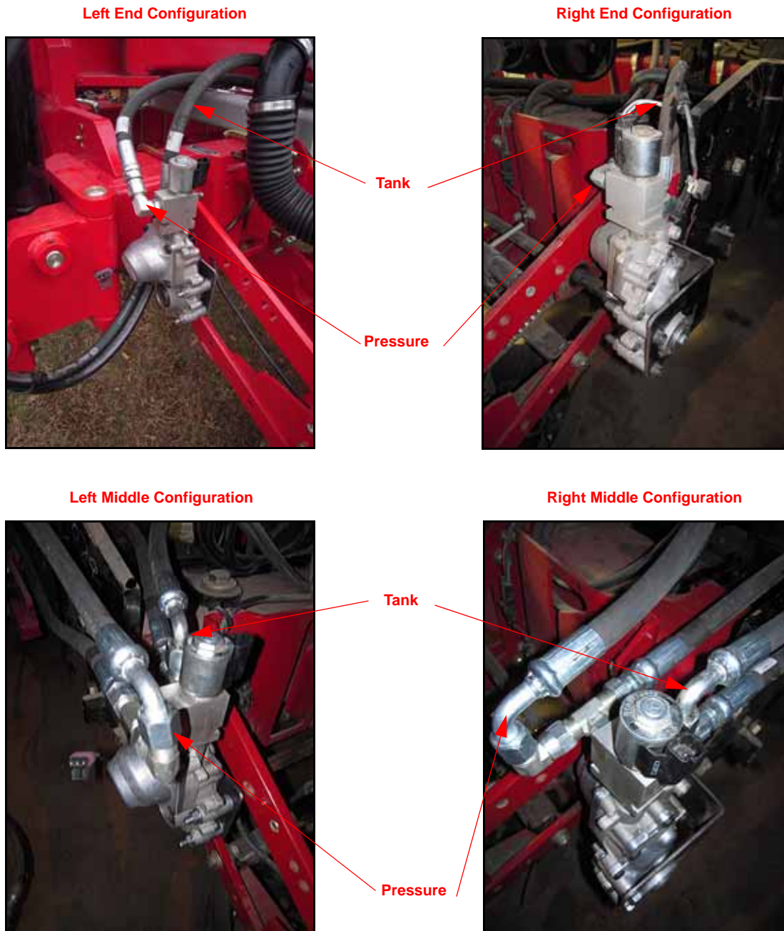
FIGURE 19. Pressure and Tank Hoses Installed
