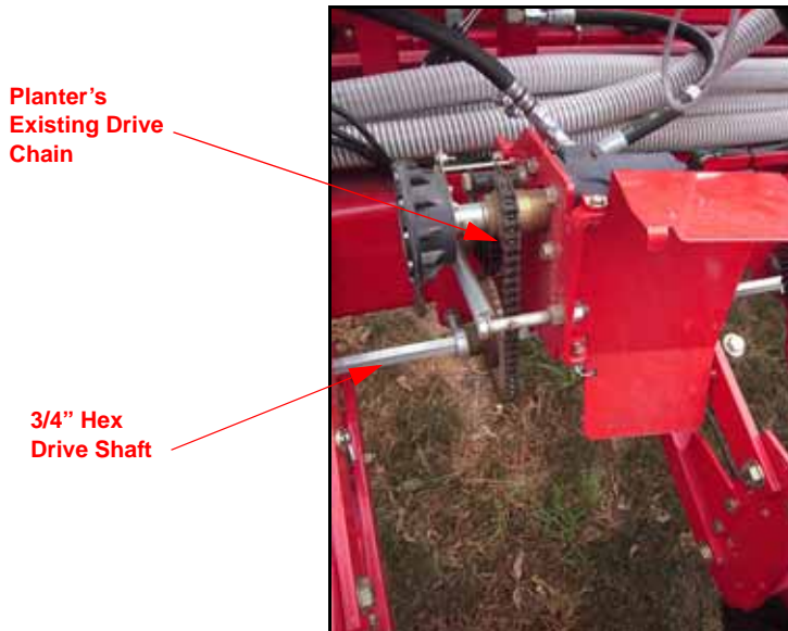
FIGURE 2. Machine's Existing Hex Shaft
