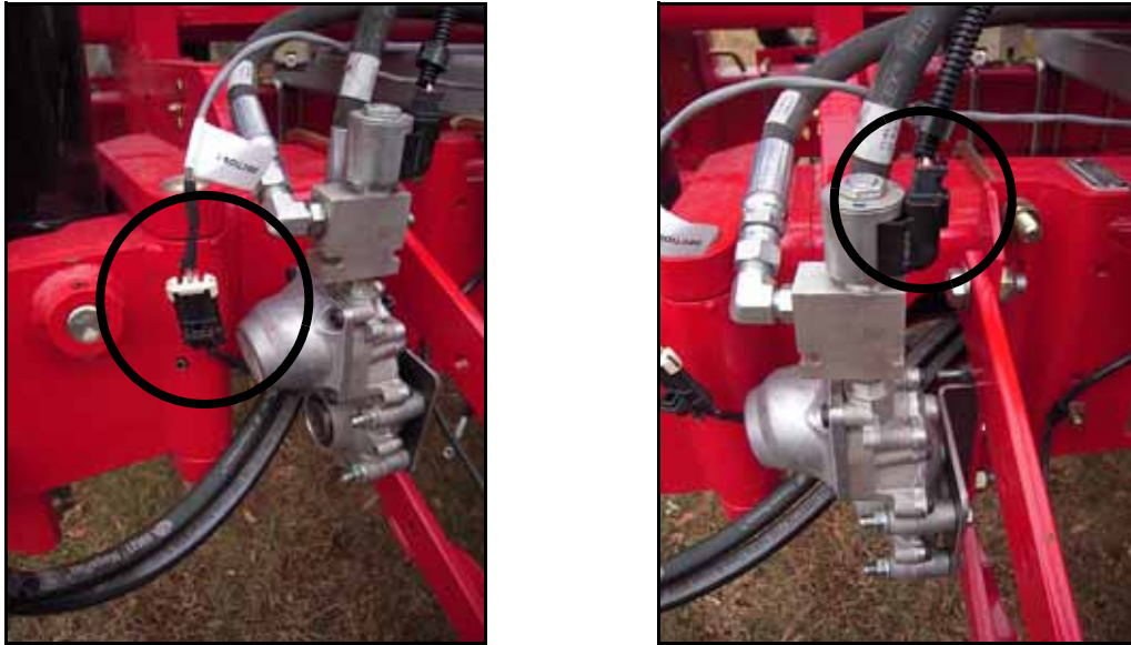
FIGURE 4. Harness Cable Connections on the Row Units
