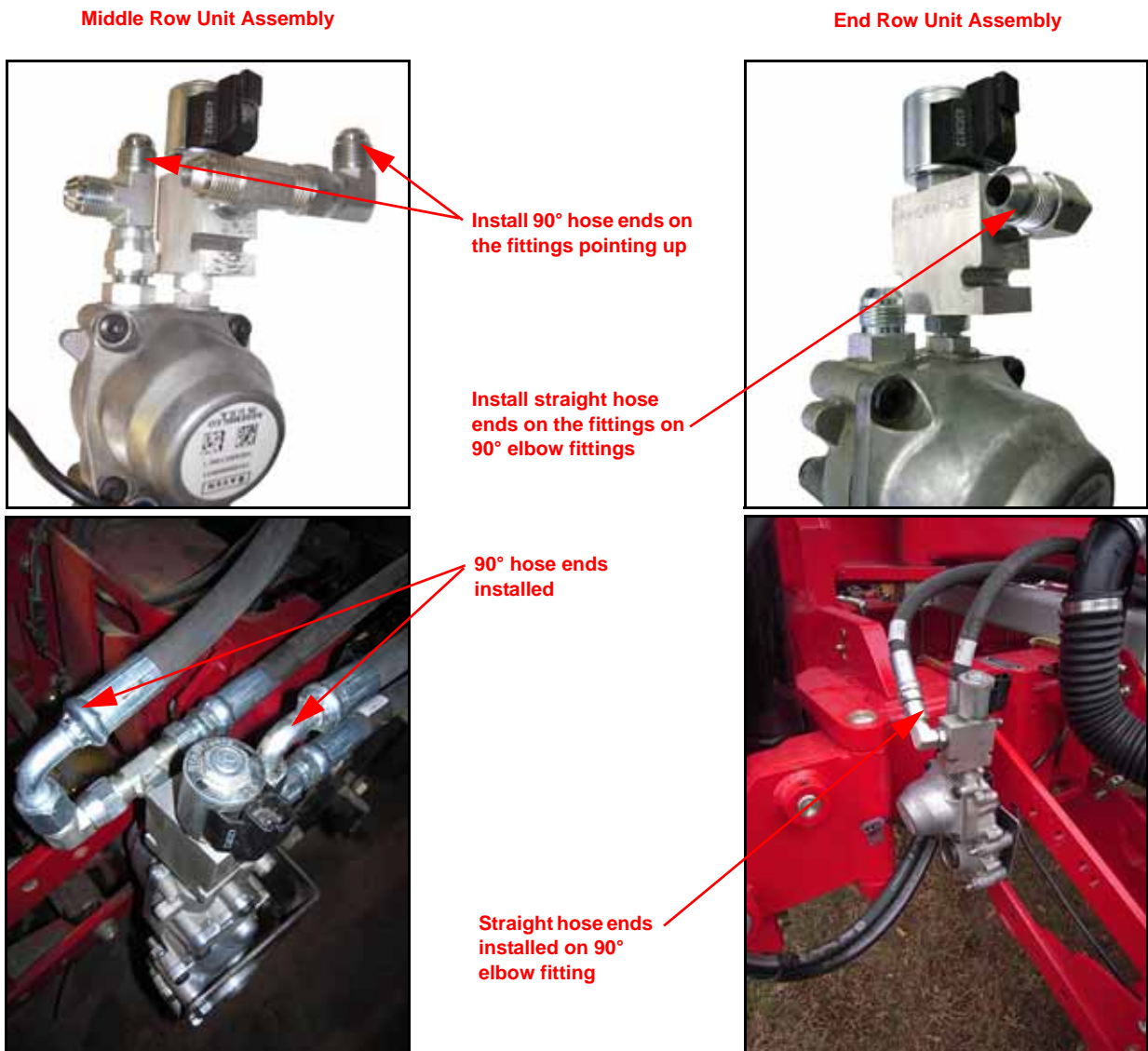
FIGURE 18. Hose Installation Illustration
