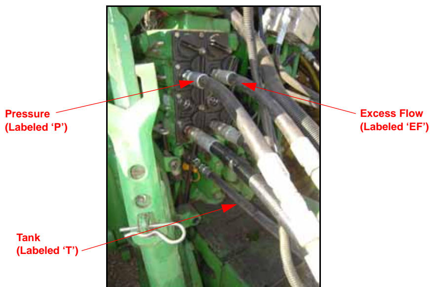
FIGURE 22. Hydraulic Hoses Connected to the Tractor
