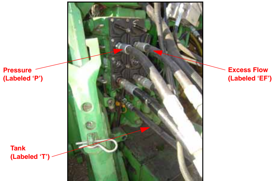
FIGURE 24. Hydraulic Hoses Connected to the Tractor
