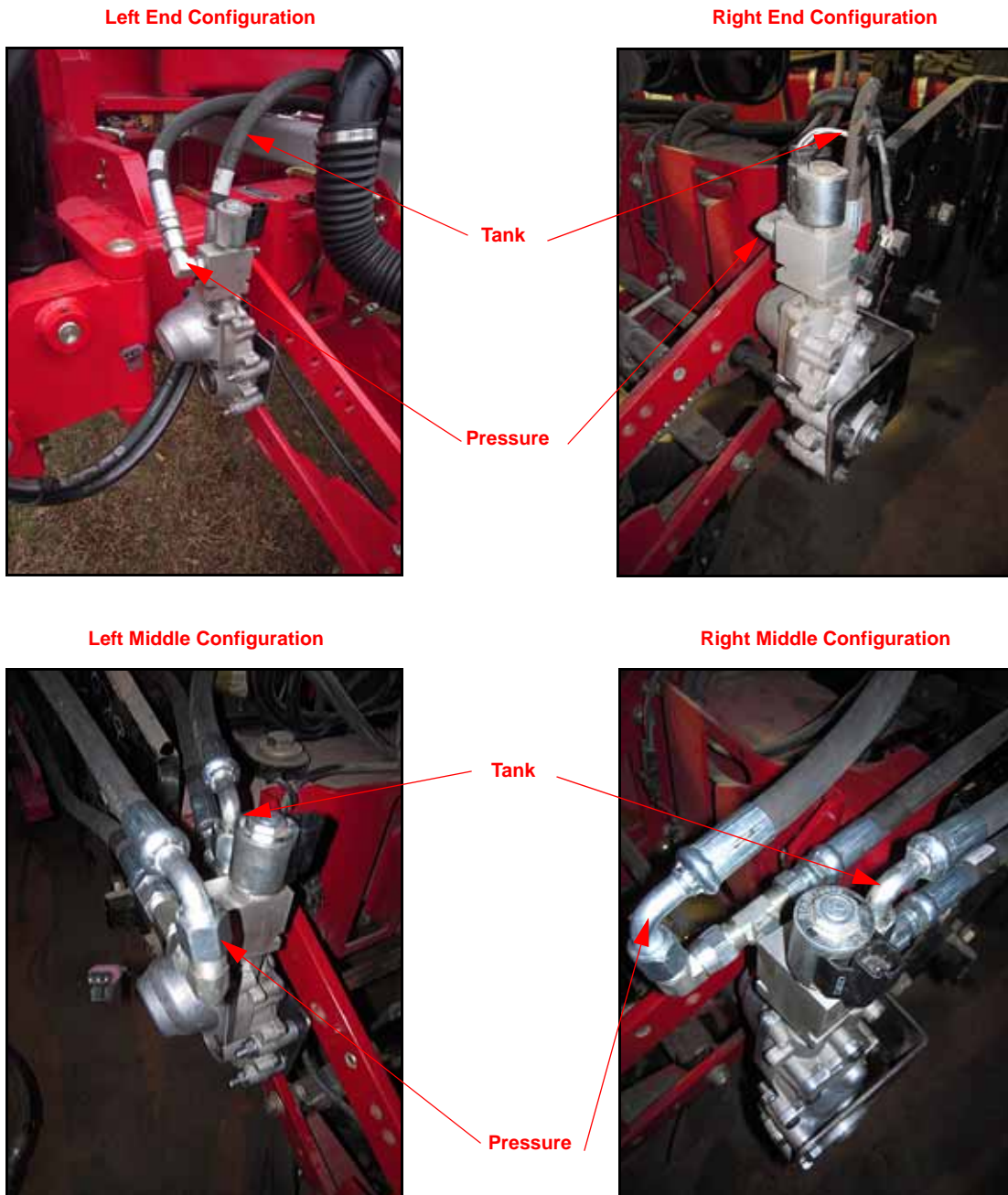
FIGURE 20. Pressure and Tank Hoses Installed
