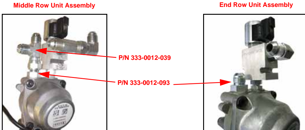
FIGURE 7. PWM Valve and Fittings Installed
