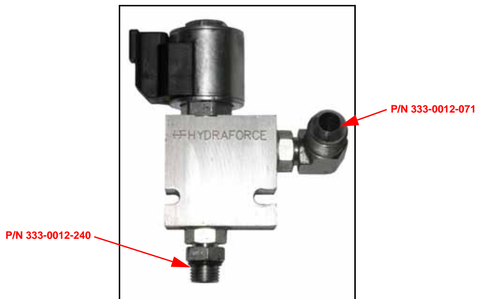
FIGURE 5. Fittings and PWM Valves Installed - End Row Units
