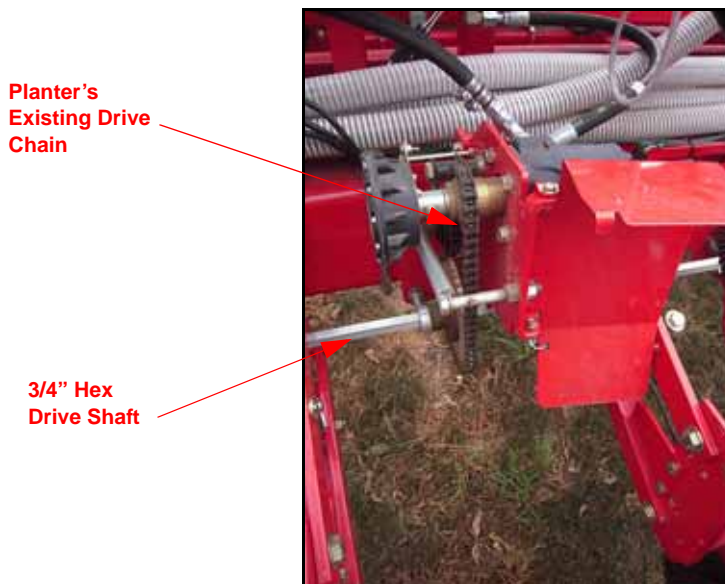
FIGURE 2. Machine's Existing Hex Shaft
