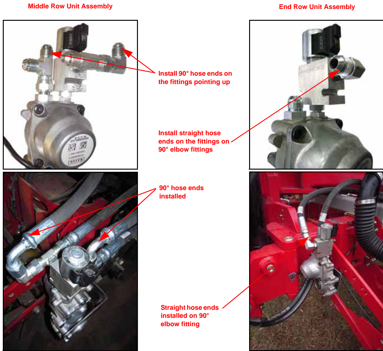
FIGURE 19. Hose Installation Illustration
