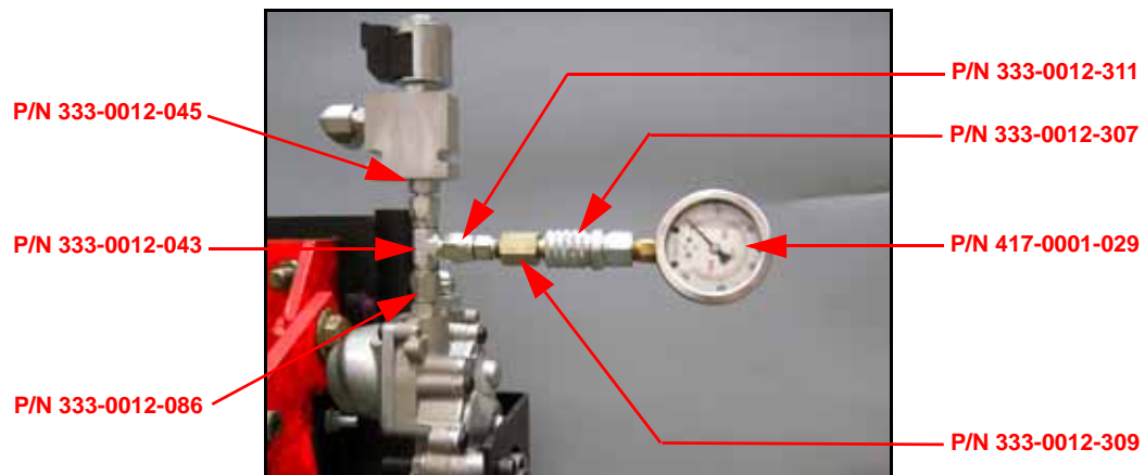
FIGURE 15. Mounted Pressure Gauge Test Kit
