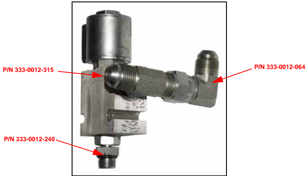
FIGURE 6. Fittings Installed PWM Valve - Middle Row Units
