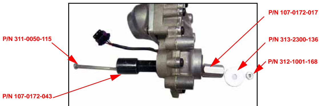
FIGURE 8. Drive Coupler Assembly
