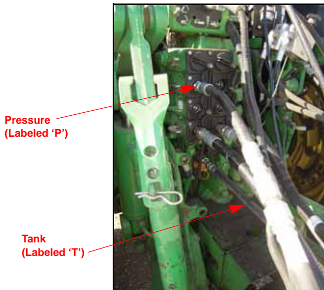
FIGURE 25. Hydraulic Hoses Connected to the Tractor
