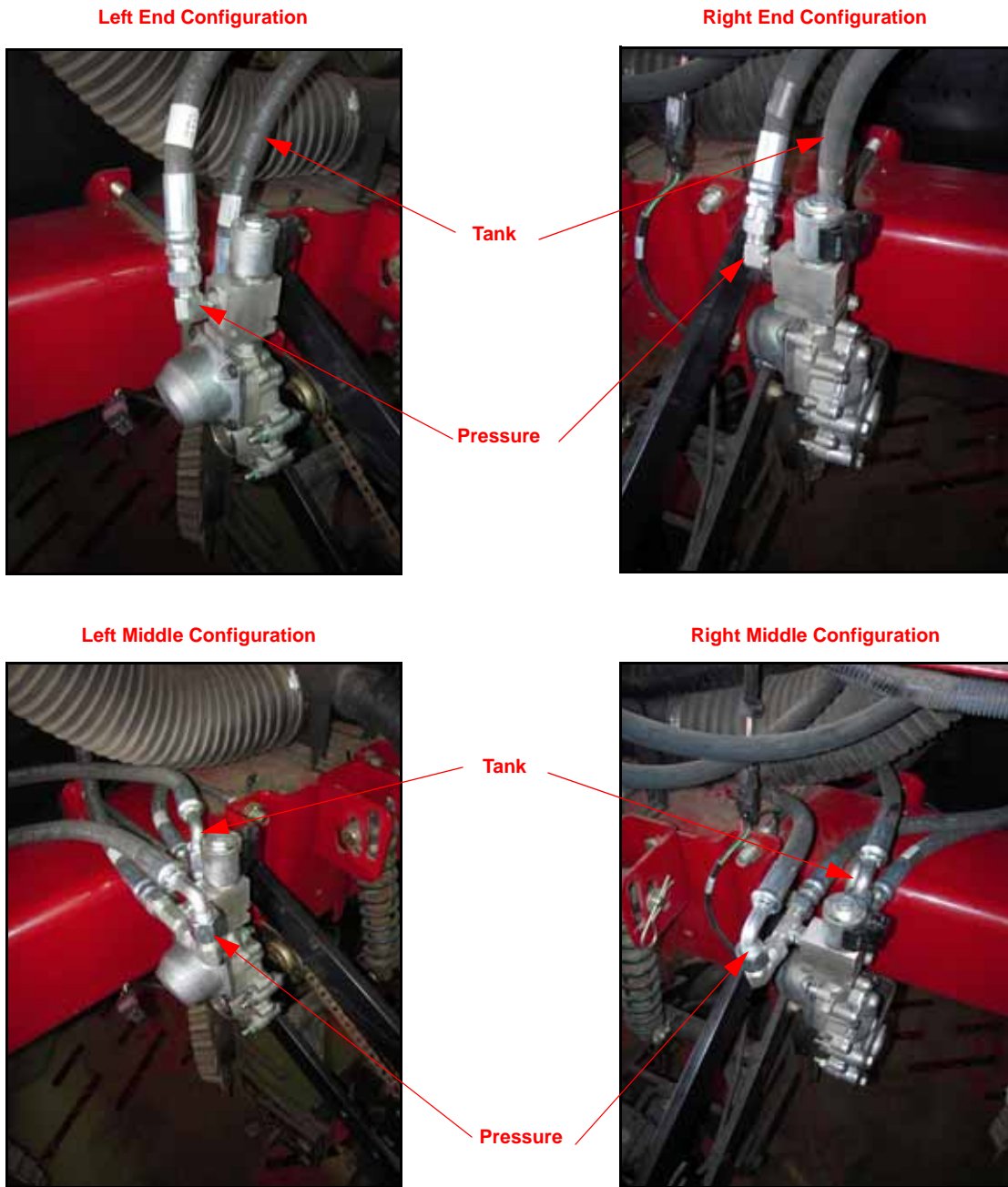
FIGURE 16. Pressure and Tank Hoses Installed
