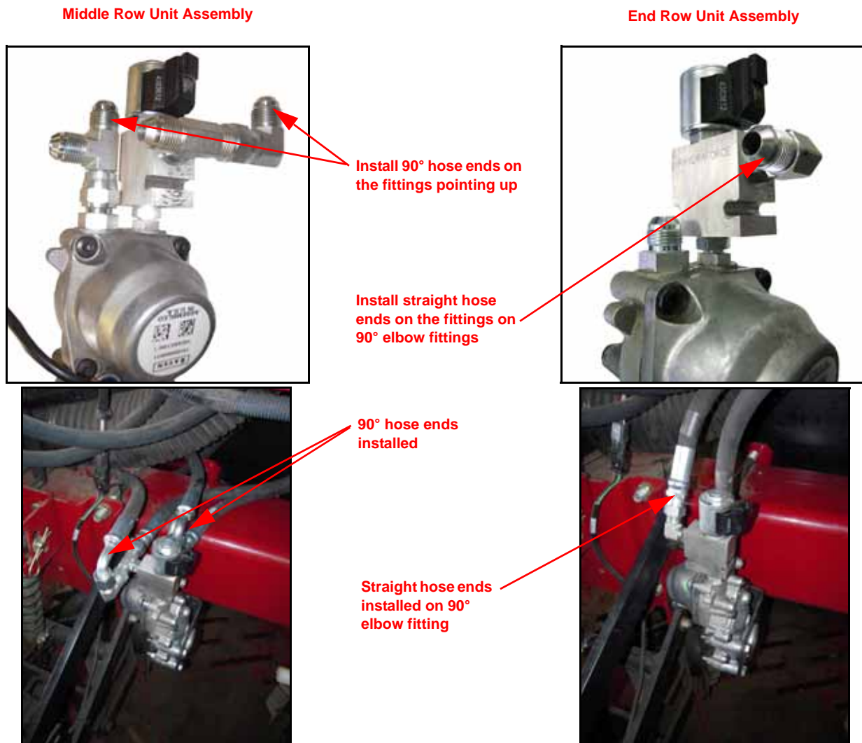
FIGURE 15. Hose Installation Illustration
