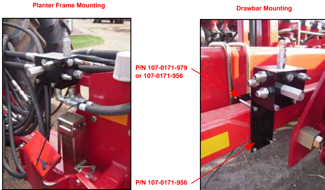
FIGURE 14. OmniRow Hydraulic Valve Installed
