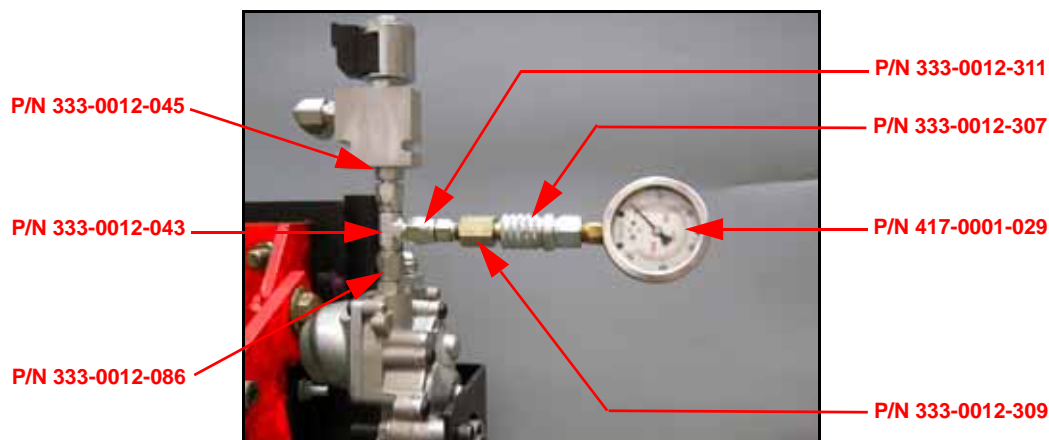
FIGURE 12. Mounted Pressure Gauge Test Kit
