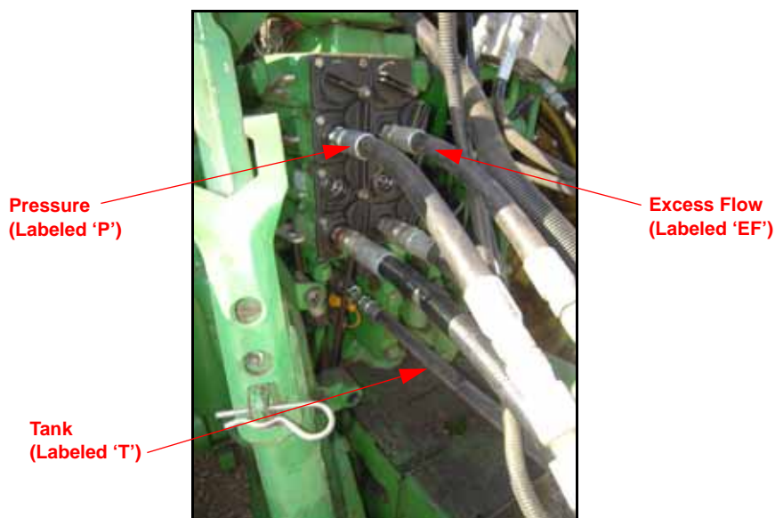
FIGURE 19. Hydraulic Hoses Connected to the Tractor
