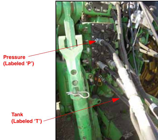
FIGURE 20. Hydraulic Hoses Connected to the Tractor
