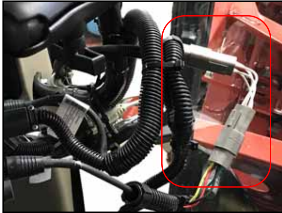
FIGURE 9. CAN Bridge Cable Connected to HDU Harness Cable
