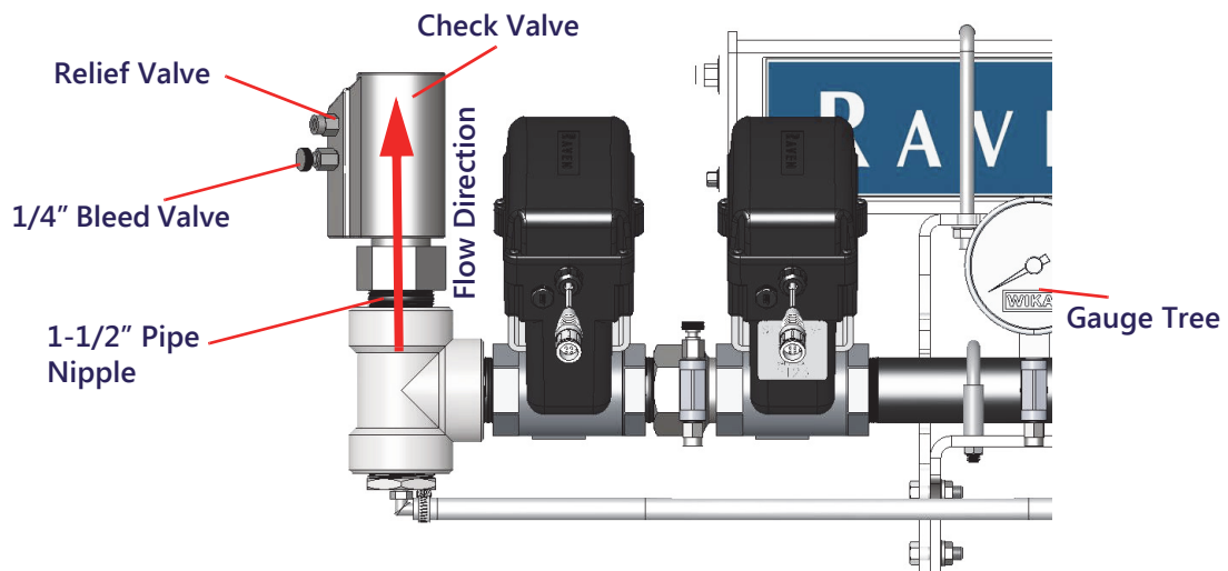
FIGURE 2. Installed Check Valve Assembly
