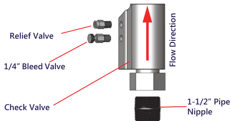
FIGURE 1. Multi-Section Check Valve Assembly
