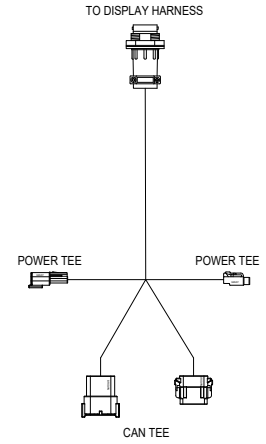
CABLE, RS1, CASE IH MAGNUM, LARGE FRAME 115-4010-085 * USE WITH MAGNUM/NH T8 2015 & NEWER
