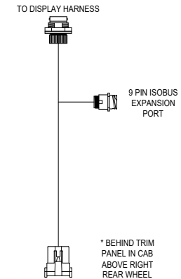
CABLE, ISOBUS DISPLAY ADAPTER, AGCO TRACTORS 115-7300-142 * USE WITH MF 86X0/87XX CHALLENGER MT 600C/D/E
