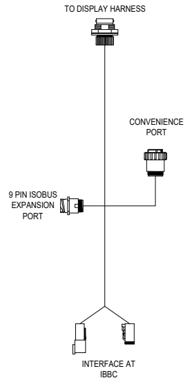
CABLE, CAN/PWR, OEM ISO TO RAVEN ISO BULKHEAD 115-7300-022
